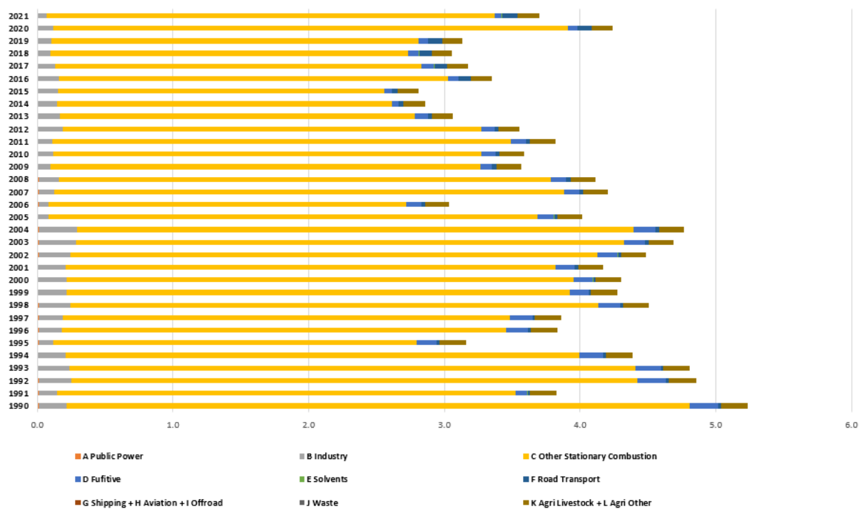
Figure 85. Distribution of benzo (k) fluoranthen between sectors for period 1990 – 2021.
