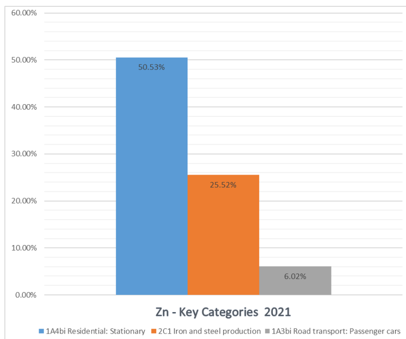
Figure 71. Key Categories assessments of Zn emissions for 2021
