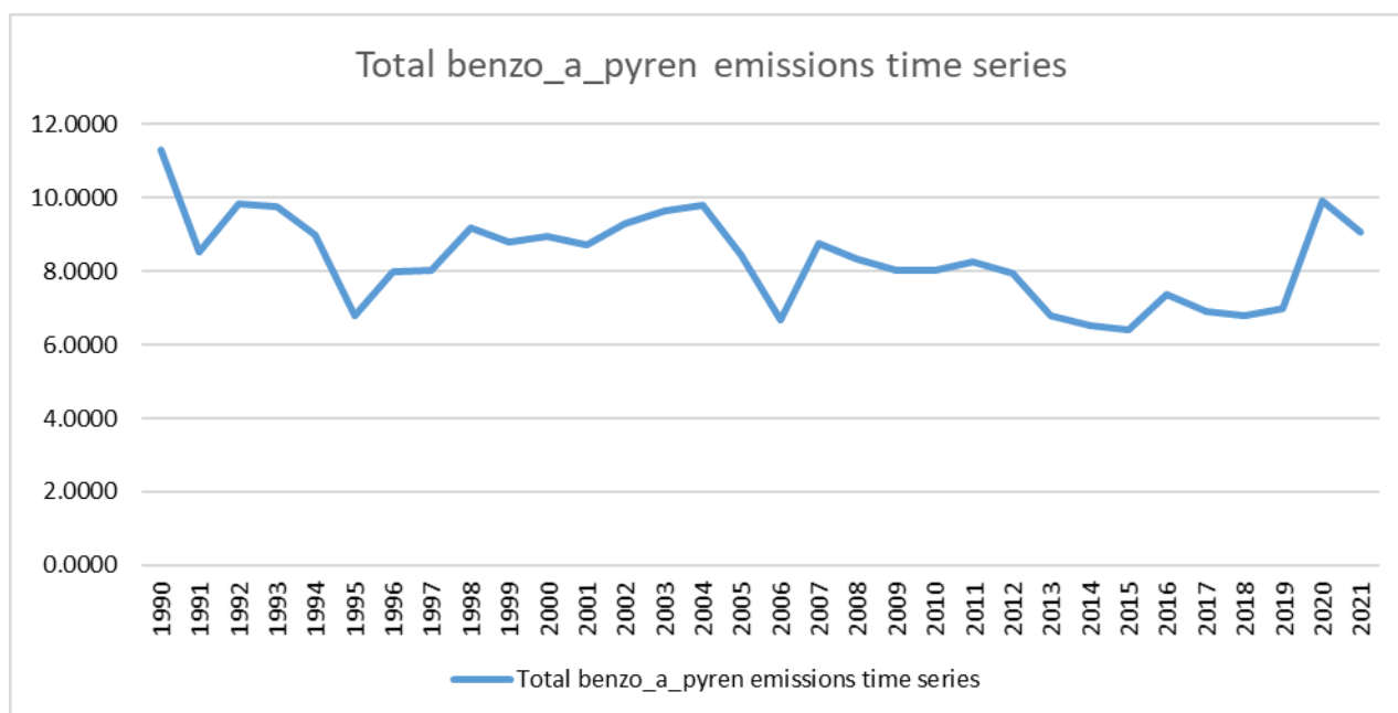
Figure 78. Total benzo a pyren emissions time series from 1990 to 2021.
