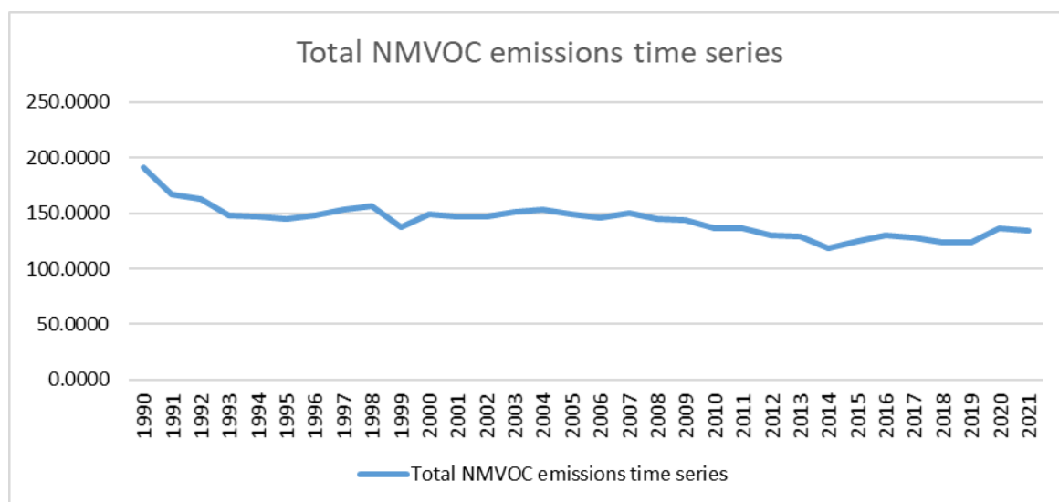
Figure 6. Total NMVOC emissions time series from 1990 to 2021.
