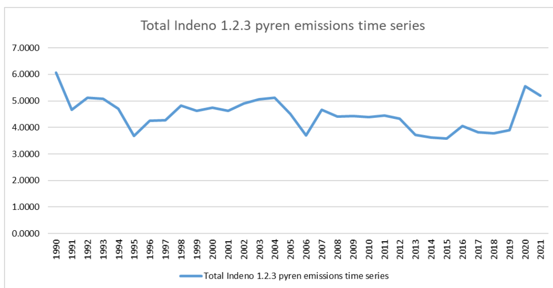
Figure 90. Total Indeno 1,2,3 pyren emissions time series from 1990 to 2021.
