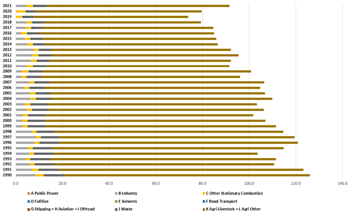
Figure 13. Distribution of NH 3 between sectors for period 1990 – 2021
