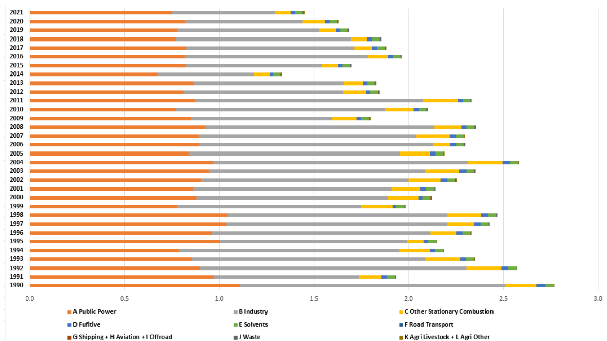
Figure 45. Distribution of Hg between sectors for period 1990 – 2021
